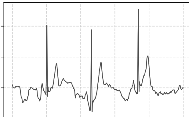
Sample 1
