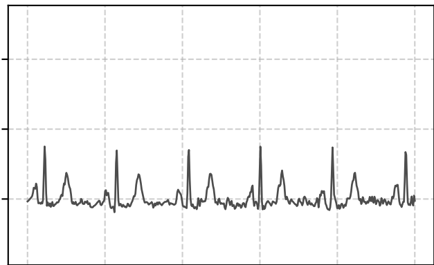
Sample 0
