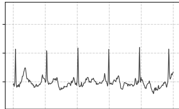
Sample 2
